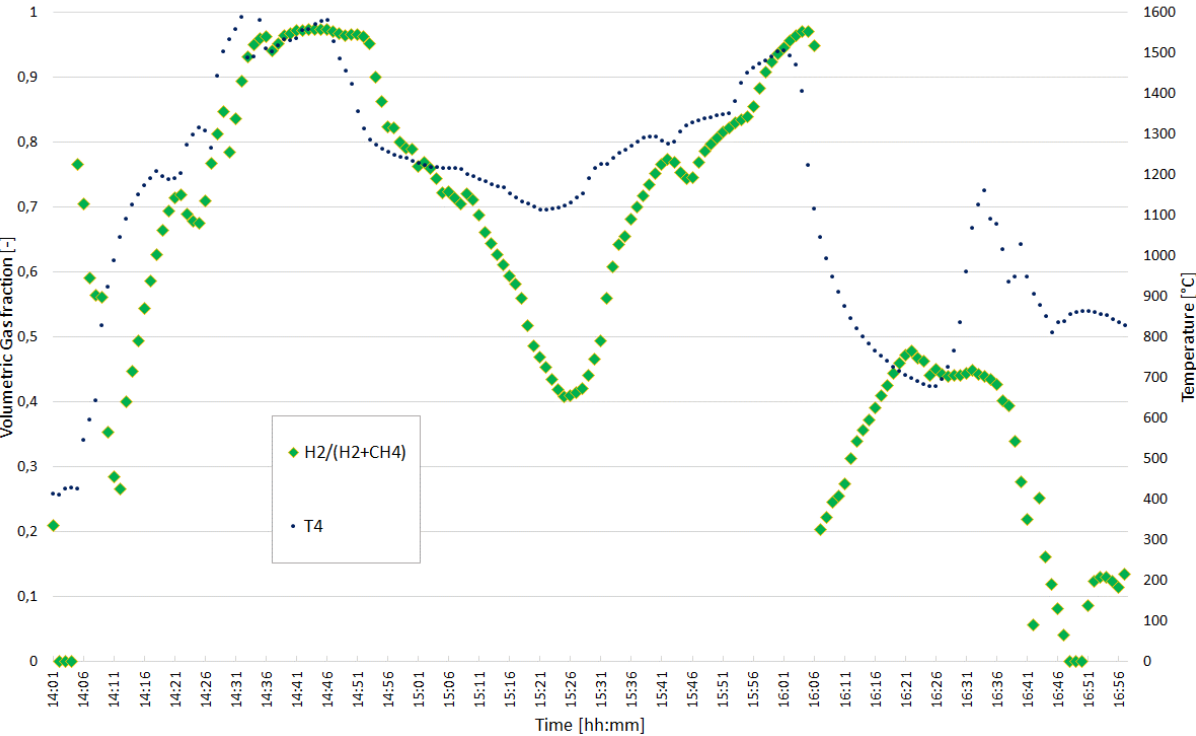
Figure 6: Ratio of H 2 to (H 2 +CH 4 ) dependent on temperature, Test V3.3
