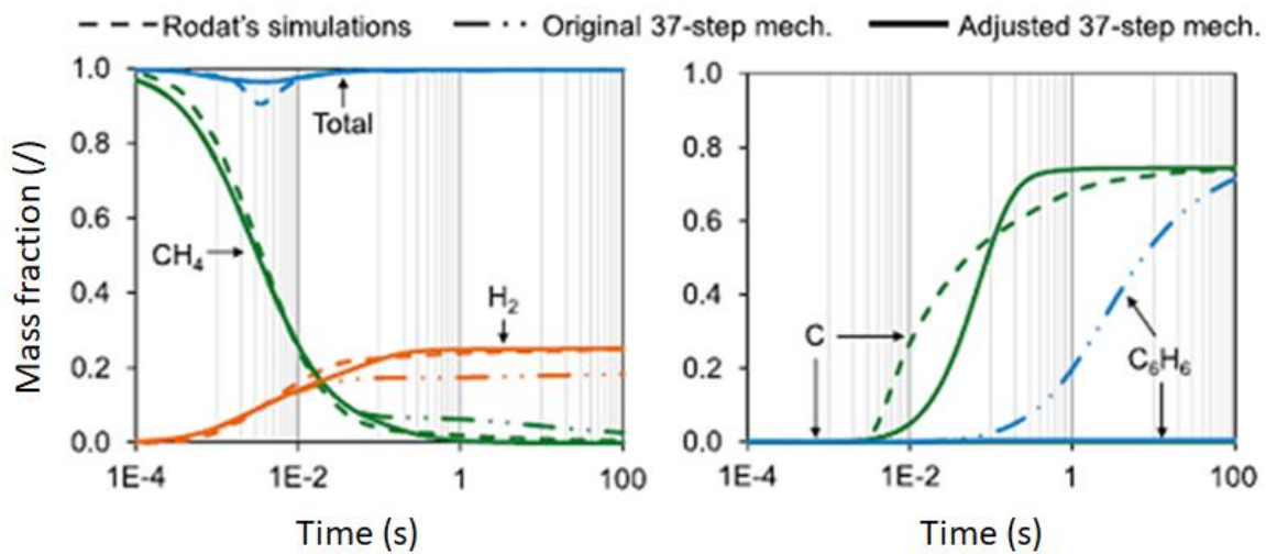
Figure 2: Thermal decomposition of Methane at 1700 K [5]
