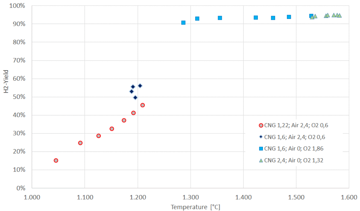
Figure 7: Hydrogen yield as a function of temperature (CNG/Air/O 2 in m 3 STP /h) [8]
