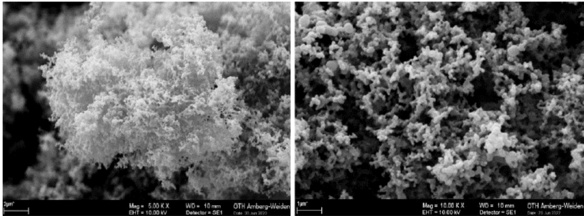
Figure 9: REM photos of soot, with 5.000 and 10.000 enlargement [8]
